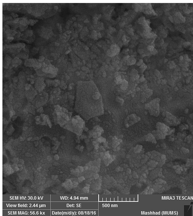
Fig. 4. FESEM image of prepared CNPs in 500 °C (S2).
