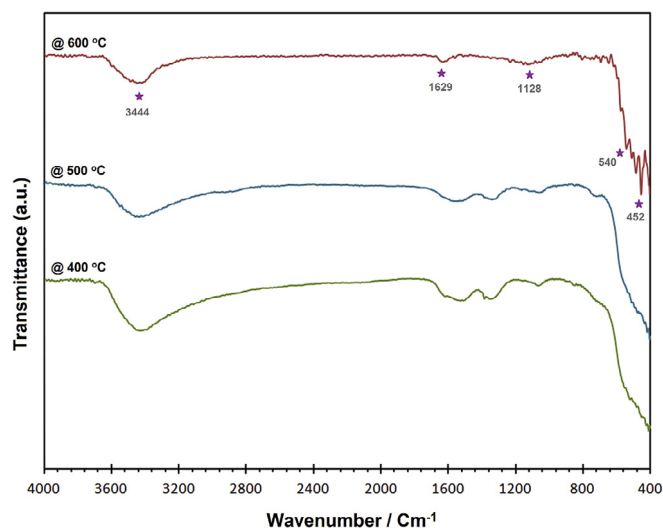
Fig. 5. FTIR spectra of calcined CNPs in various temperatures.
