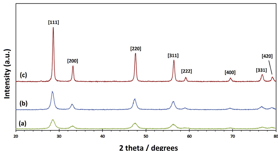
Fig. 3. XRD patterns of calcined CNPs in different temperatures; (a) 400, (b) 500, and (c) 600 °C.
